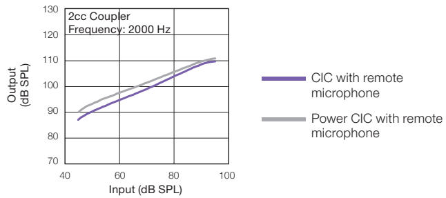
Input/Output response
